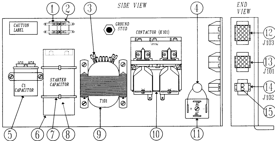
POWER PANEL SIDE VIEW
